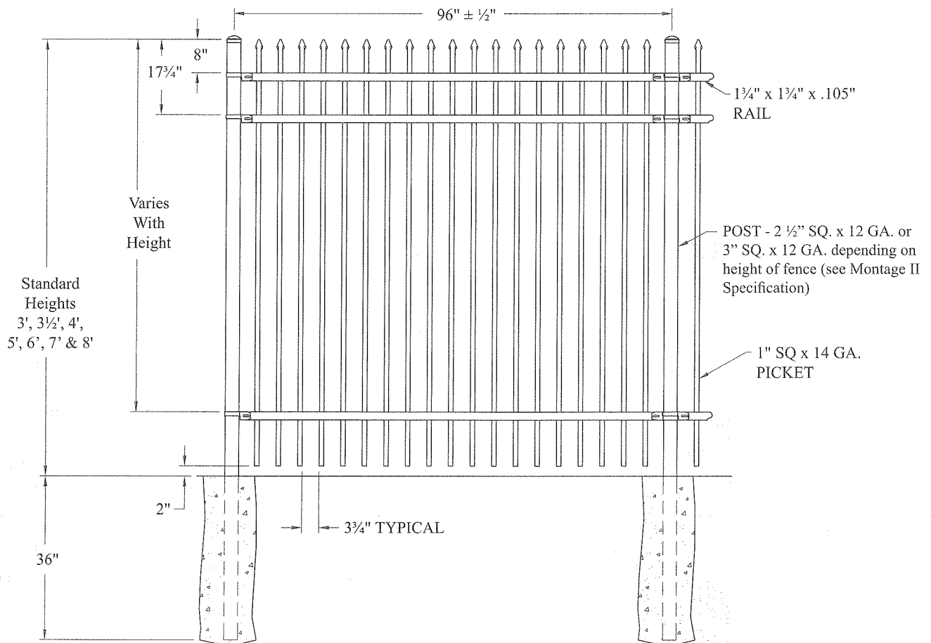
TYPICAL PANEL DRAWING (Classic Style shown; Genesis, Majestic & Invincible also available)
